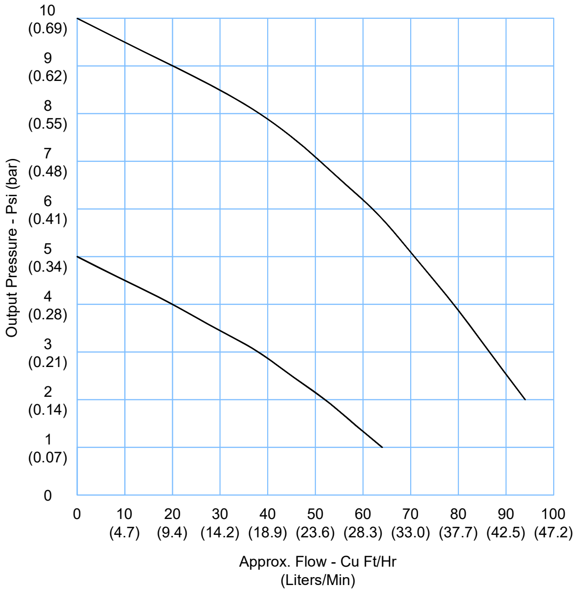
R-900 or R-920 (Supply Pressure = 30 Psi)
