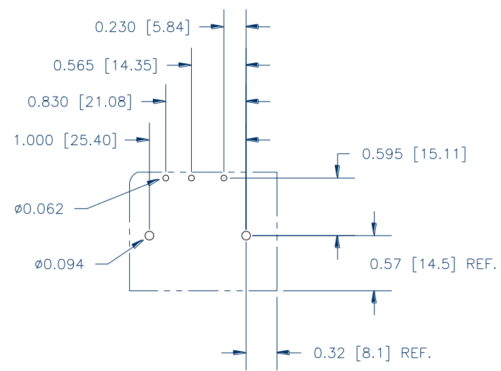
CIRCUIT BOARD FOOTPRINT
