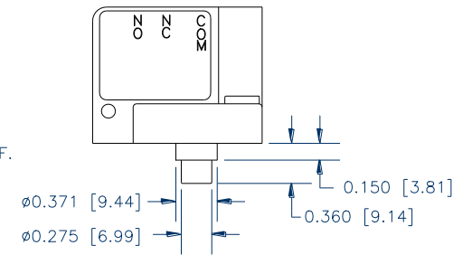
MANIFOLD MOUNT
