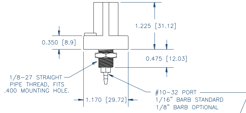
PANEL MOUNT
